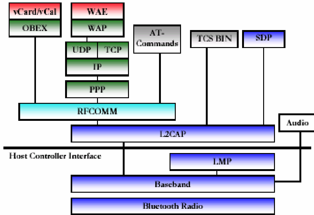
Figure 1 The Bluetooth Protocol Stack [Ana01]
