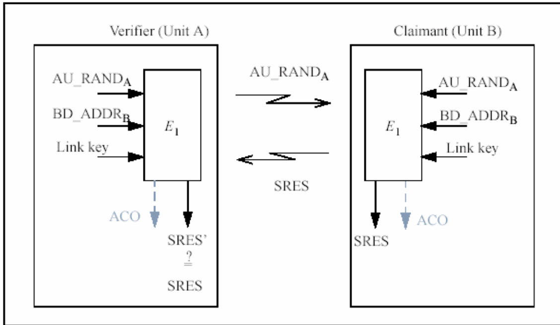
Figure 2 Challenge-Response for Bluetooth [Tra00]
